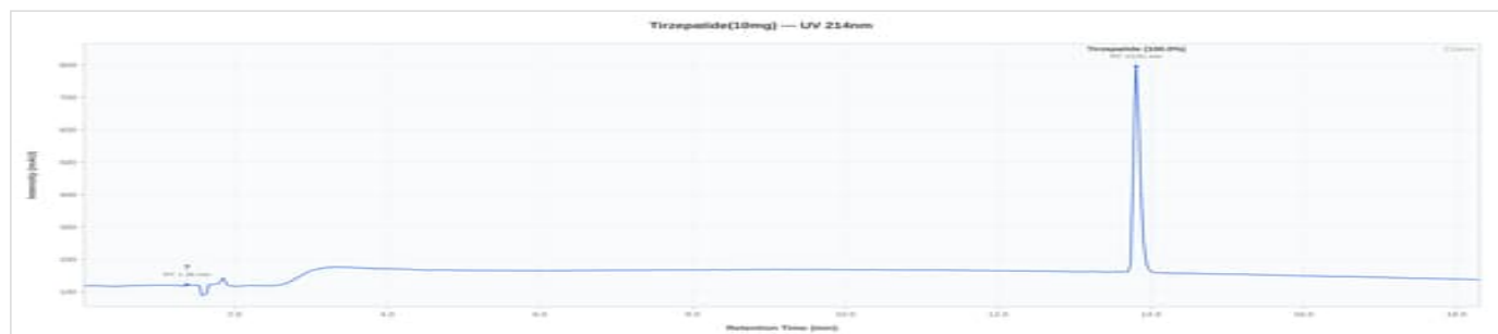
Tirzepatide 10mg - LOT-2026-800-10-1S: UV Chromatogram
