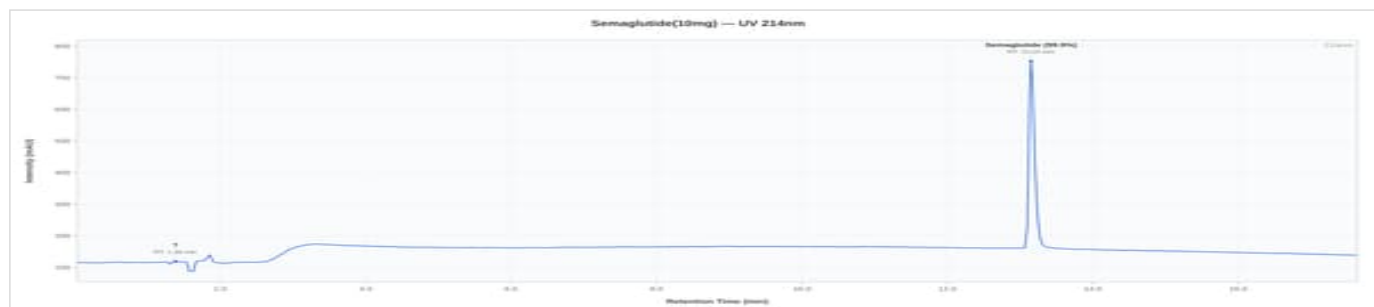
Semaglutide 10mg - LOT-2026-700-10-1S: UV Chromatogram
